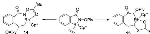
Figure 1. Regiochemical preferences in alkene insertion.
