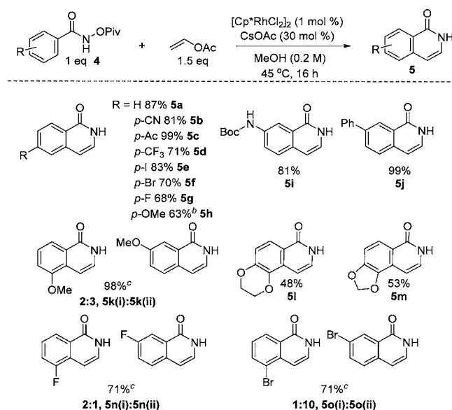
Scheme 1. Substrate Scope of the C–H Activation/Annulation with Vinyl Acetate a,b
